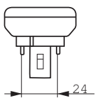
GX24d-2
