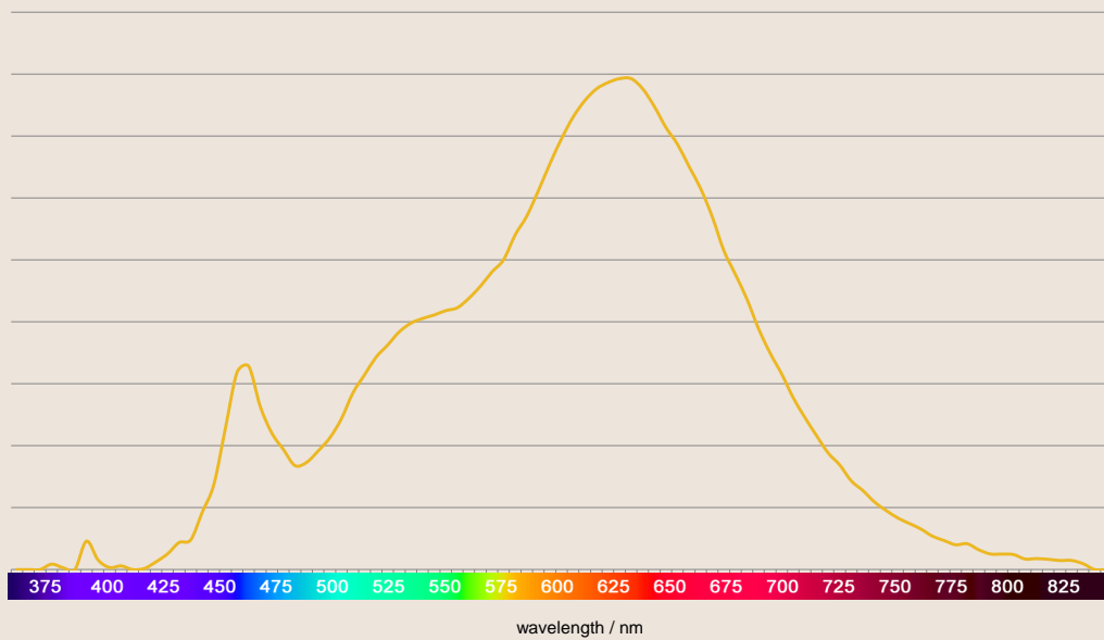
SPECTRAL POWER DISTRIBUTION OF LEDON 5W P45
