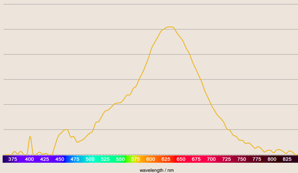
SPECTRAL POWER DISTRIBUTION OF LEDON 1.5W G4
